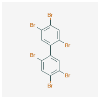
Figure 1: Example of one isomeric structure of HBB (CASRN 59080-40-9) [9], [10].
