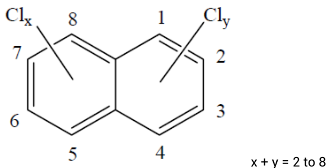
Figure 3: General chemical structure of a PCN congener [70].
