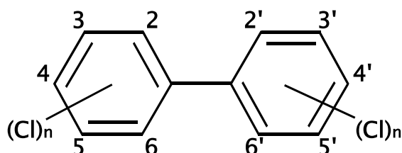
Figure 2: General chemical structure of a PCB congener [67]. Each side of the carbon ring structure can have 1-5 chlorine atoms attached
